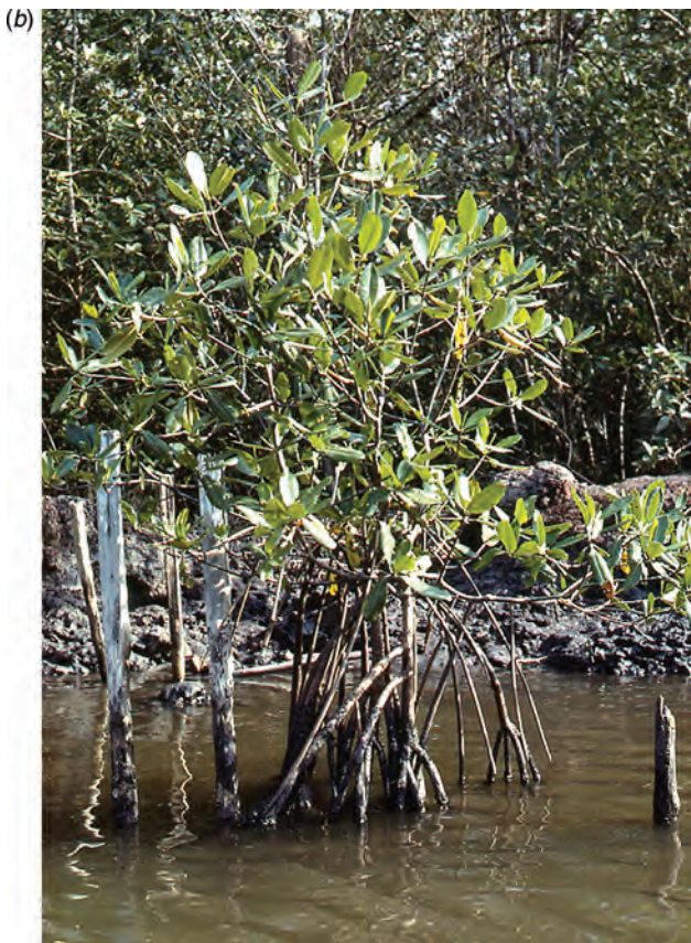
FIGURE 1.3 Swamps. (a) Floodplain swamp (Ottawa River, Canada). (b) Mangrove swamp (Caroni wetland, Trinidad).
